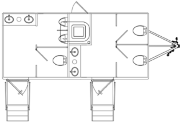
Model: WC8182-2F1M 8'W x 18'L Capacity: 475 Gallons
